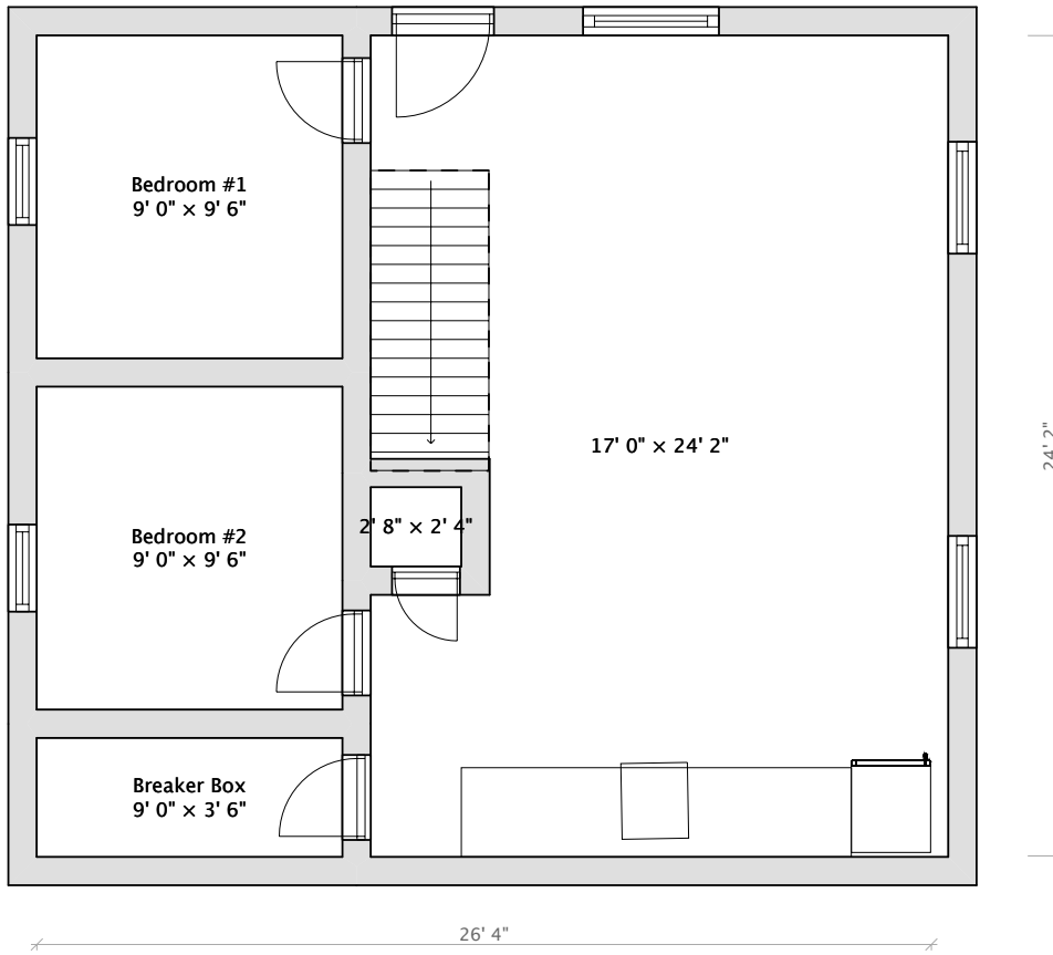
321 D E Merry First Floor
